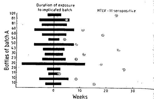
Fig 1—Relation between time of infusion of batch A, number of vials transfused, and development of anti-HTLV-III.
